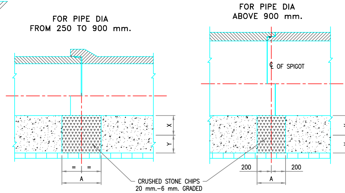
LONGITUDINAL SECTIONS FOR RCC PIPES AT JOINT
