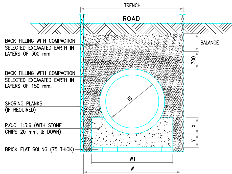
RCC (NP3) BEDDING CROSS SECTION
