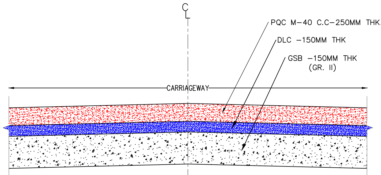
TYPICAL CROSS-SECTION OF RIGID PAVEMENT.
