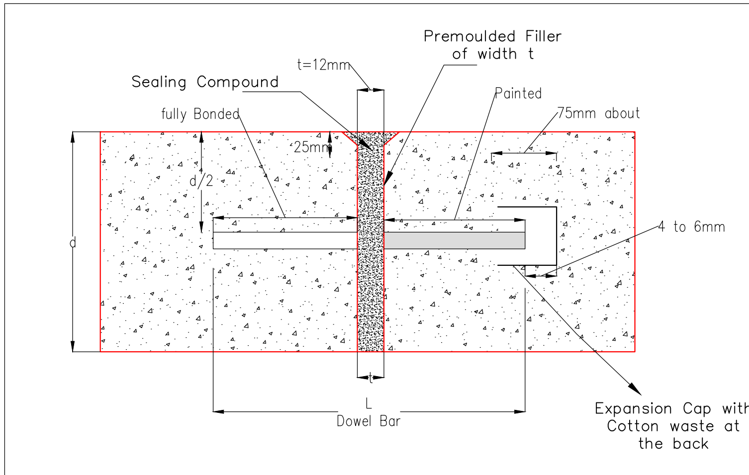
TYPICAL CROSS-SECTION OF EXPANSION JOINT
